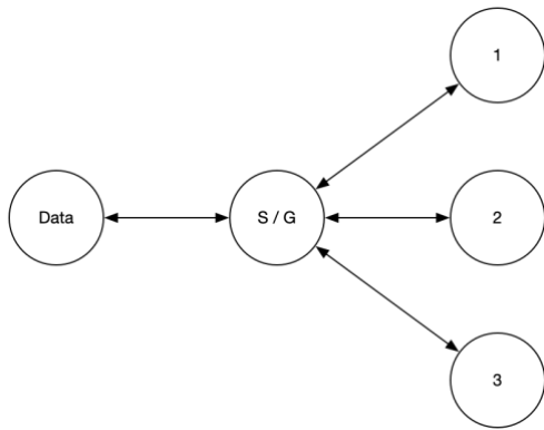
Figure 4: A demonstration of the scatter / gather pattern
