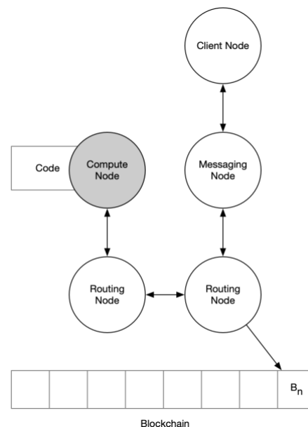
Figure 13: Code will live on compute nodes not the blockchain
